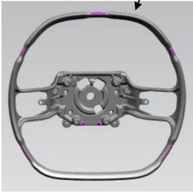
Steering Wheel and Steering Column Mount-Magnesium Alloy
